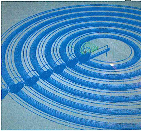
idaho's pattern was CNC milled into ash wood. this is a screenshot of the CAD milling file. #einundzwanzig #wetakeyoutomilan #einundzwanzigmilan #tortonadesignweek #fuorisonalone #germandesigncouncil #ratfuerformgebung #ratfürformgebung #idaho #cnc #cncmill
